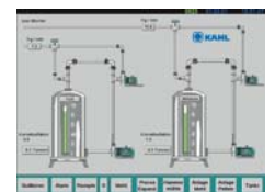
Individual tanks
